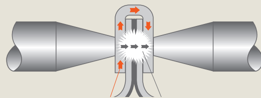
Welding a pin by electrical discharge welding
