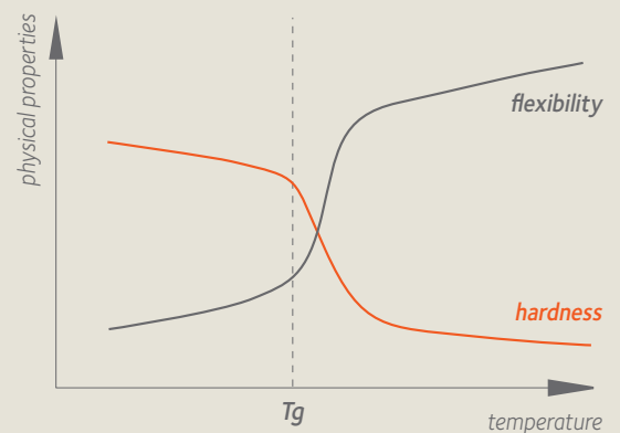
Variation in coating flexibility and hardness with temperature
